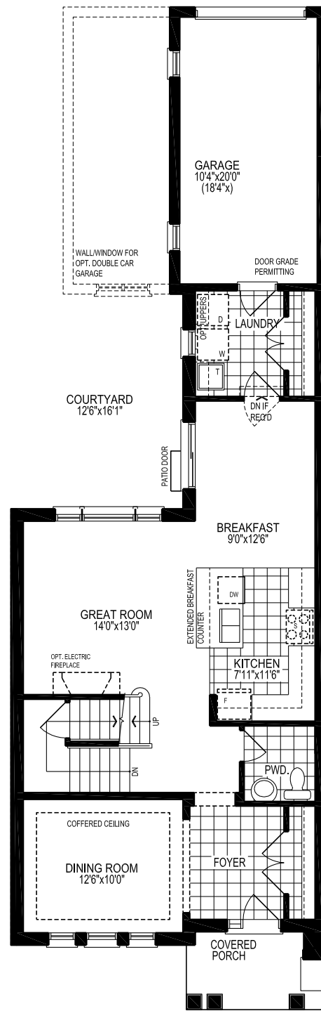
GROUND FLOOR PLAN 'A'
